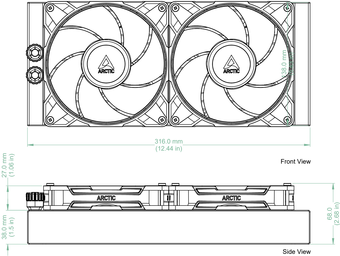
Radiator & Fans
